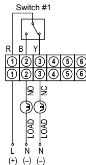
One SPDT switch Reed switches & terminal strip connection
